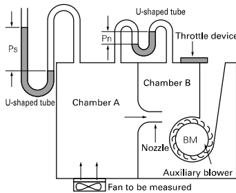
Double chamber measuring equipment
